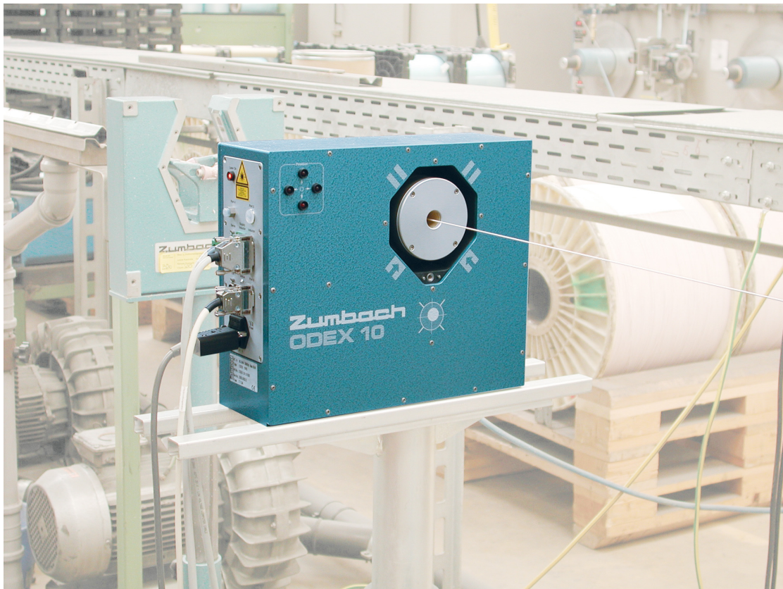
ODEX® 10 measuring unit in a jacketing line
